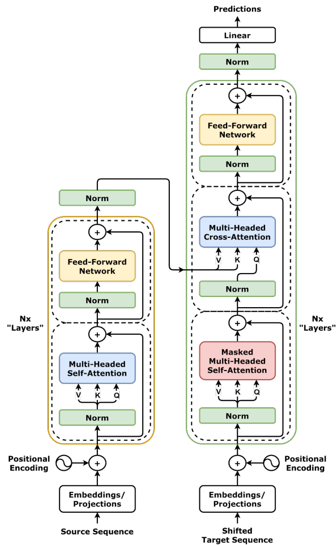
Figure 1: Transformer Architecture
